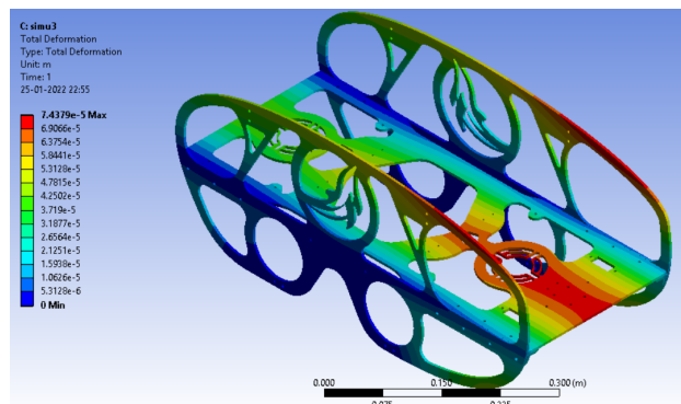
Deformation analysis of Arkaja 2.0 frame in Ansys
