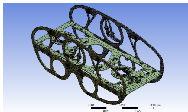
Mesh of Arkaja 2.0 frame generated in Ansys
